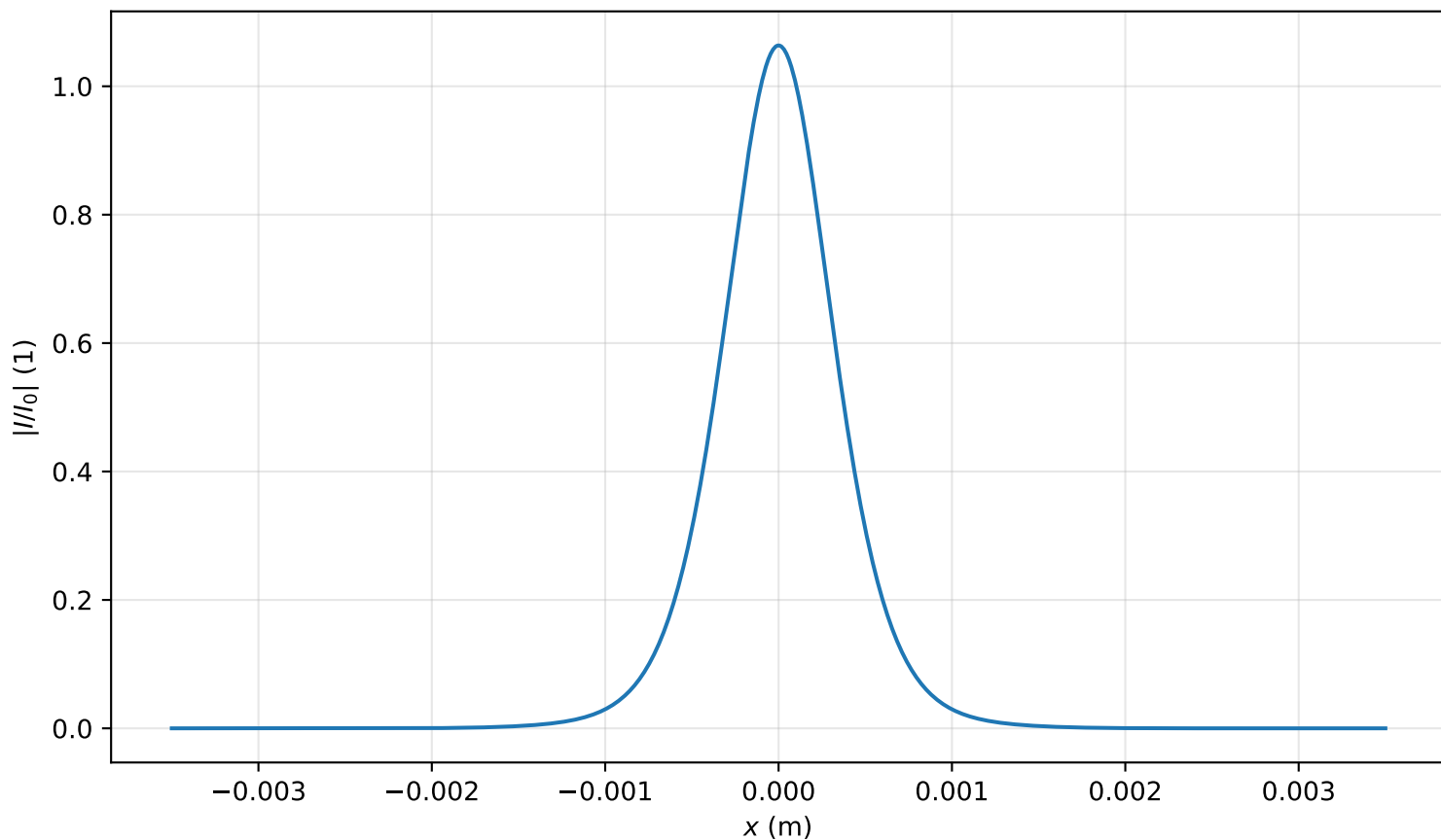
Intensity profile I(x, y = 0, z = 2.149m)/I_0 , P_{in}=0.7P_{cr} , artificial time
